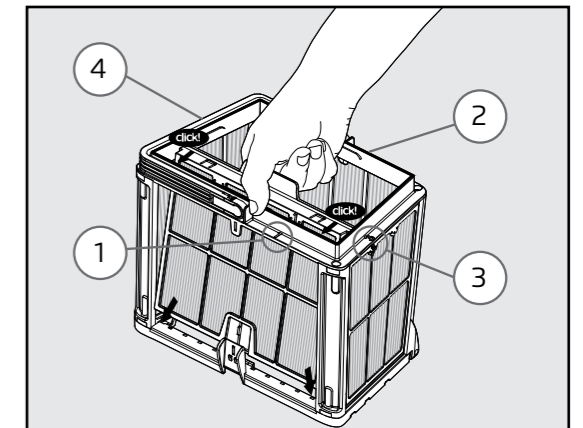
8.2.5 Reassemble the filter panels in the order 4 → 3 → 2 → 1.
