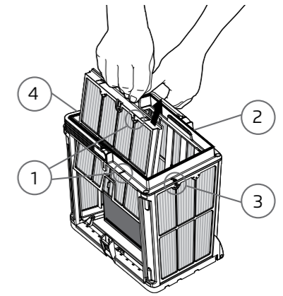
8.2.3 Continue to dismantle panels 2, 3, 4 in the same manner.
